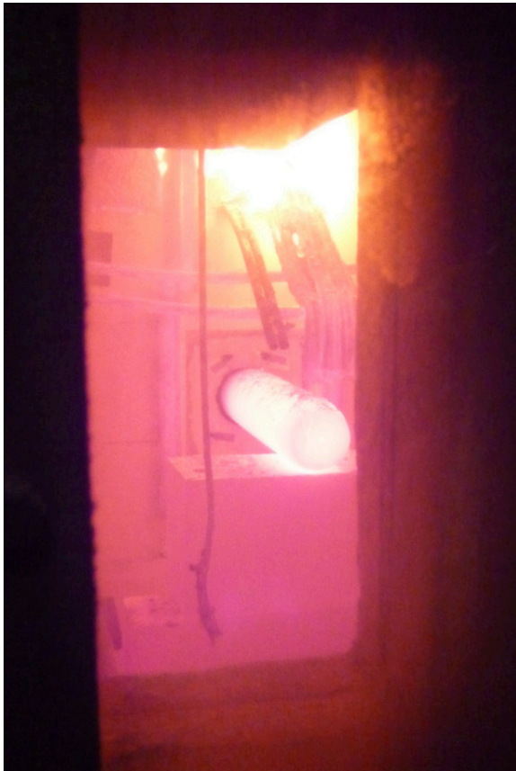
img. 5: fire test fireproof bulkhead seal
