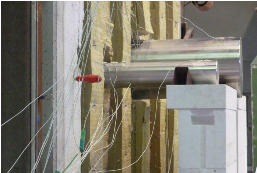
img. 3: measuring points fire test
