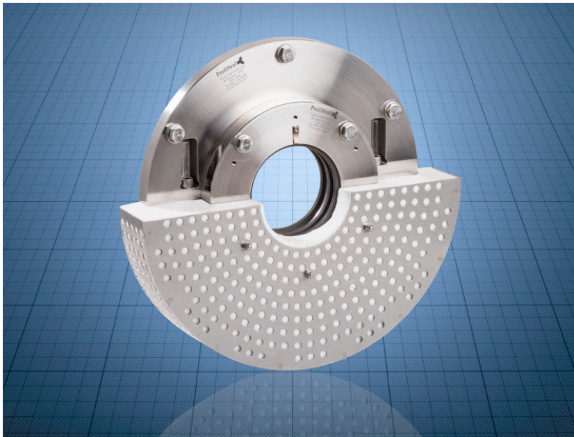
img. 1: fireproof bulkhead seal
