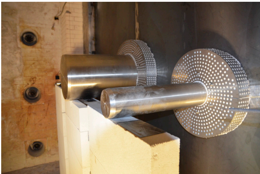
img. 4: setup fire test
